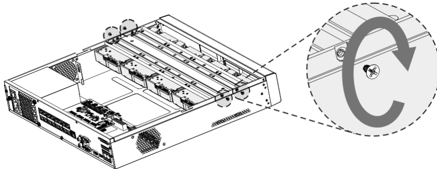
Figure 2-21 Fasten HDD bracket
