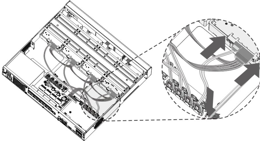
Figure 2-22 Connect cables
